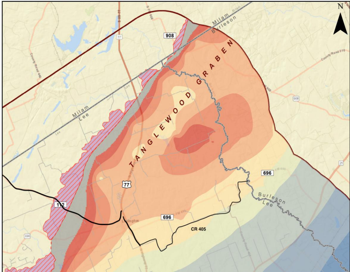
Figure 1. GMZ 1 boundaries.
